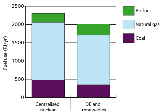
Figure 5: Total fuel use in 2023 by fuel type – baseline scenarios
